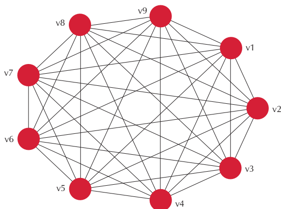
Graph 41 Complete Network
