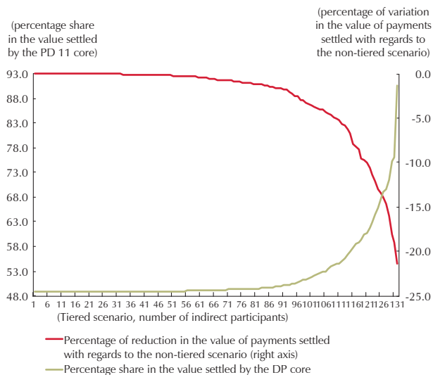
Graph 37 Concentration Risk
